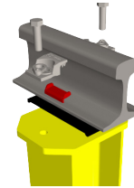
Boltable clips
